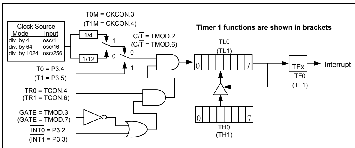
Figure 12: Timer/Counter Mode 2
