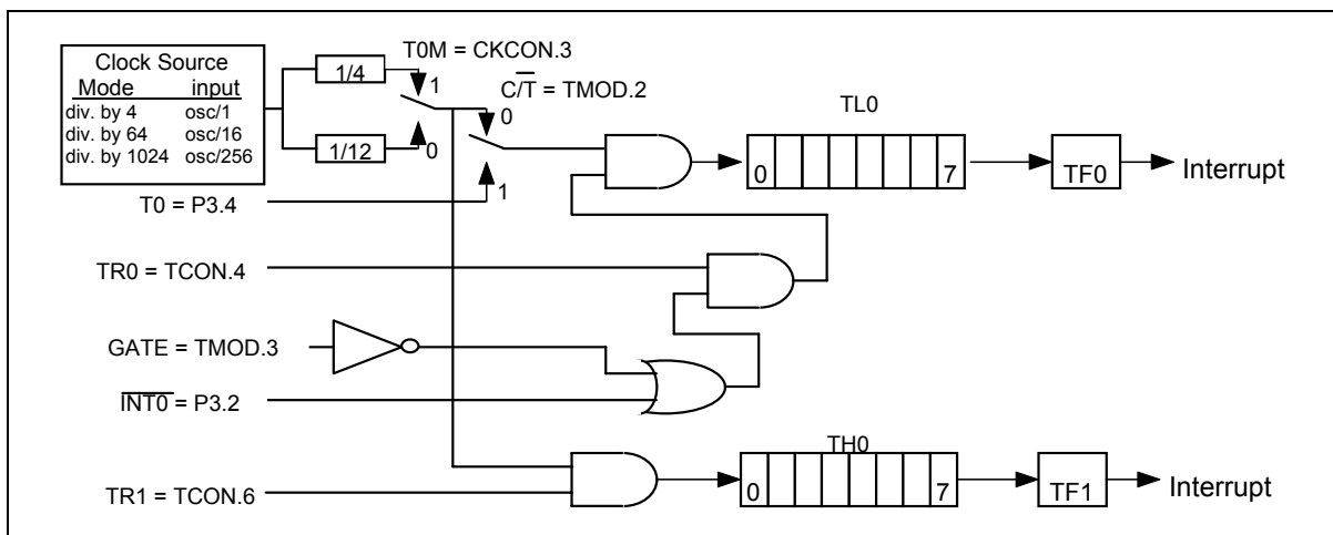
Figure 13: Timer/Counter 0 Mode 3
